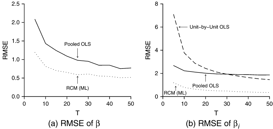
Fig. 2 Comparison of RMSE for RCM and OLS estimators of \beta and \beta_i as T varies from 5 to 50. For all runs of the experiment, N = 20 , \sigma_e^2 = 1 , and \sigma_x^2 = 0.01 . The \beta_i were drawn as \Gamma(5, 1.8^2) .
