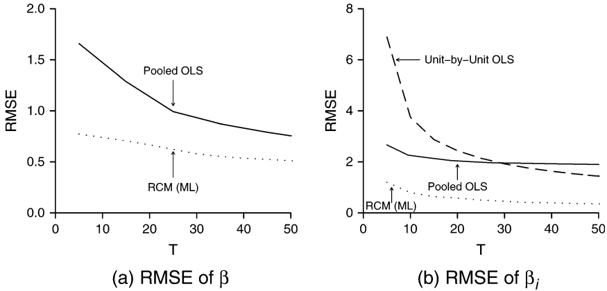
Fig. 1 Comparison of RMSE for RCM and OLS estimators of \beta and \beta_i as T varies from 5 to 50. For all runs of the experiment, N = 20 , \beta = 5 , \gamma = 1.8 , \sigma_e^2 = 1 , and \sigma_x^2 = 0.01 .
